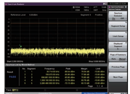
Spurious Emission
