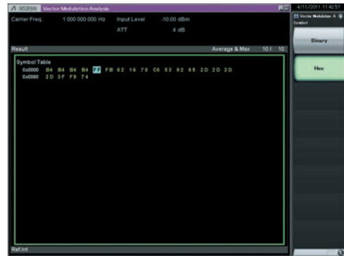
Hexadecimal example
