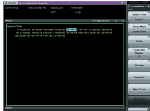
Binary example
